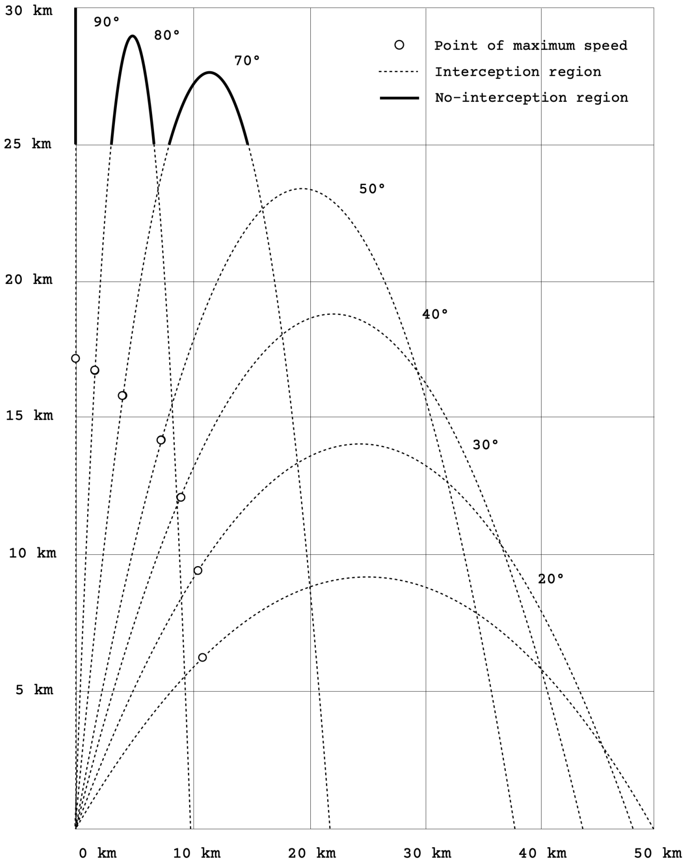
Fig.15 - RIM-66M, estimated interception envelope of CER-500TR rocket.
