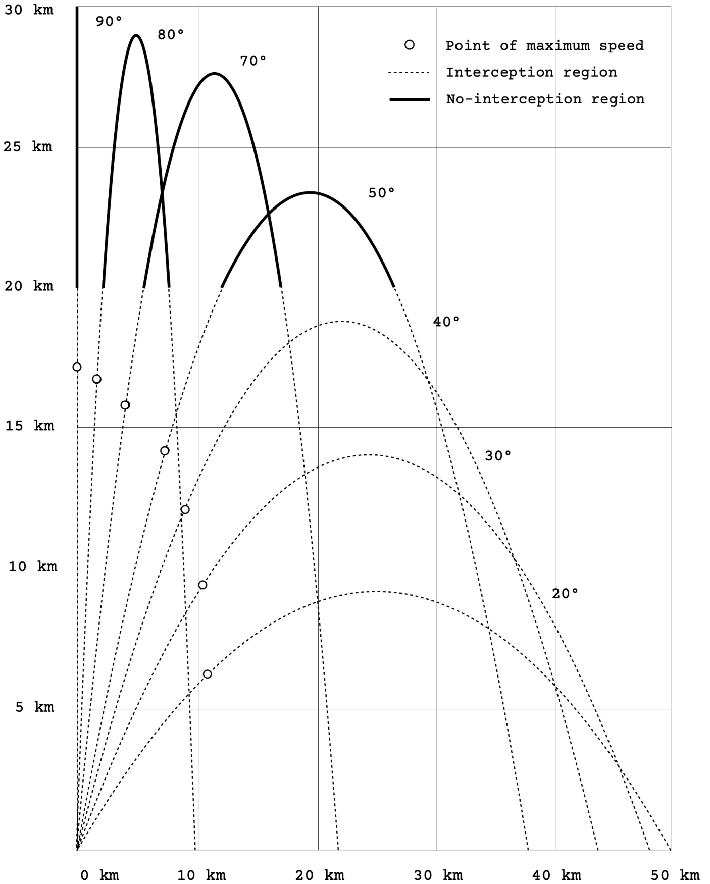
Fig.13 - MIM-23 - Hawk - Phase III, estimated interception envelope of CER-500TR rocket.
