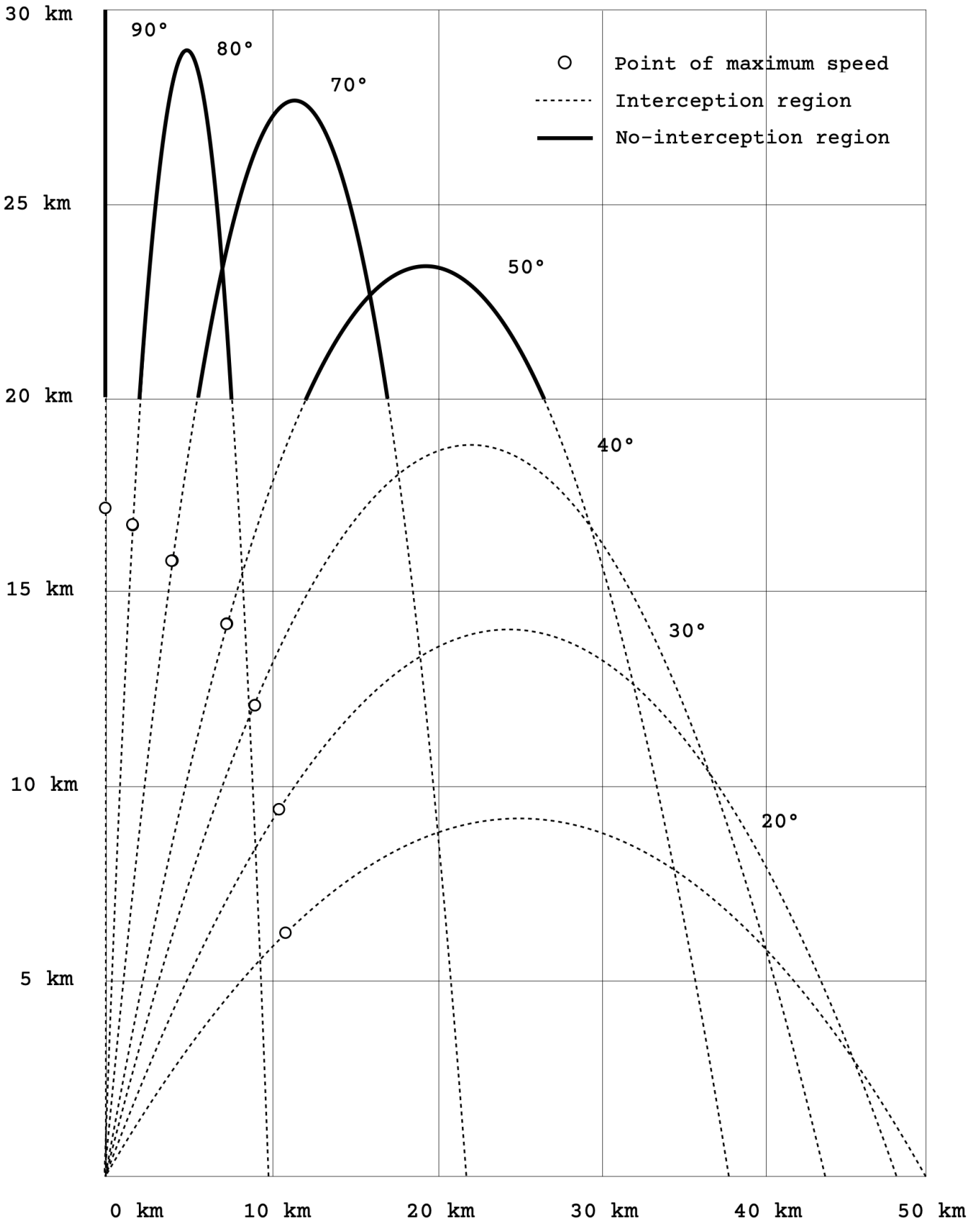
Fig.16 - 9M96, estimated interception envelope of CER-500TR rocket.
