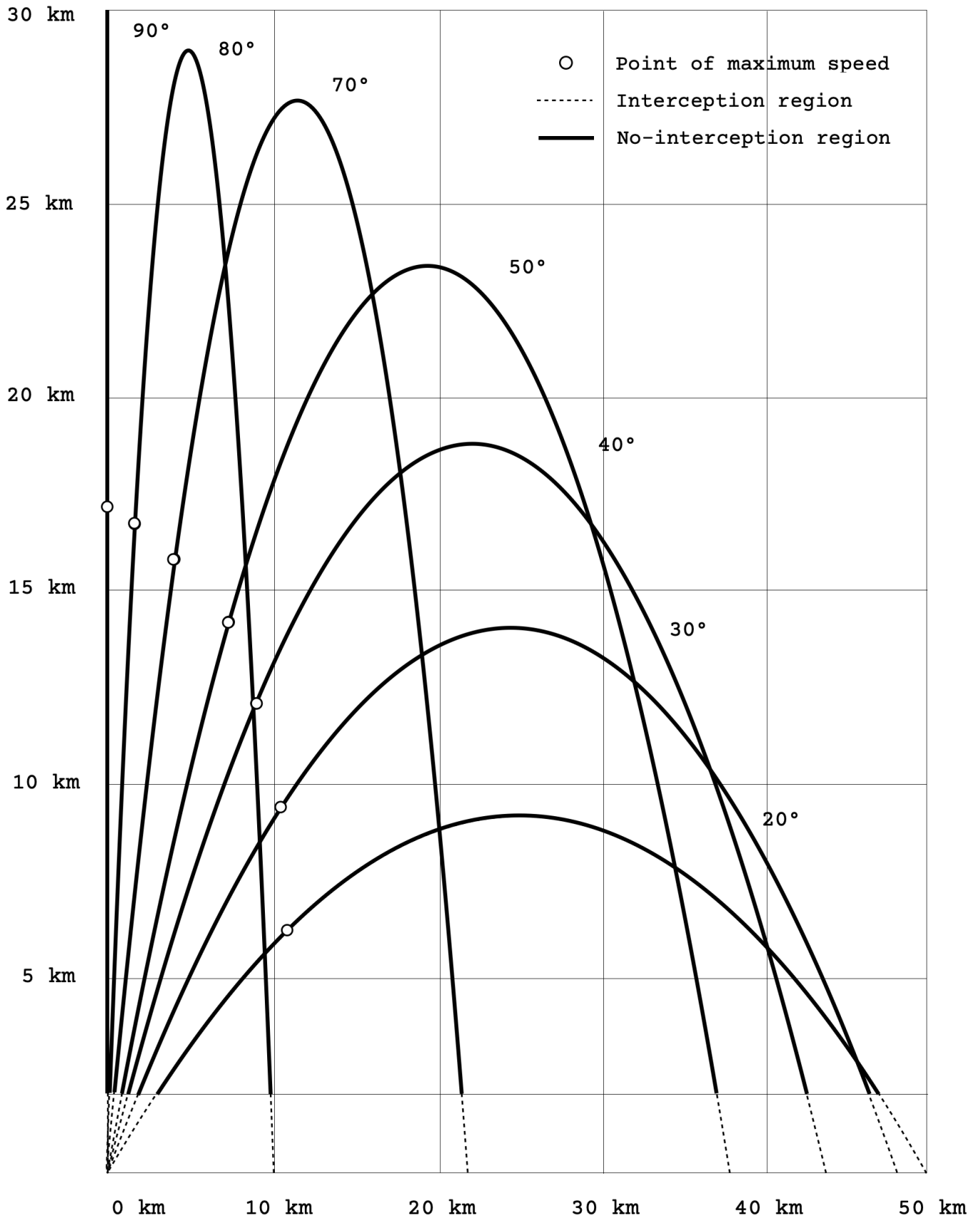
Fig.17 - Phalanx and Goalkeeper CIWS, estimated interception envelope of CER-500TR rocket.
